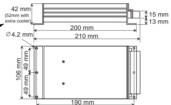
Figure 7. Dimensions with option N, wall mounting Weight: 0.91 kg with extra cooler 1.11 kg
