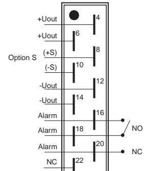
Figure 3. Alarm relay output Option -B
