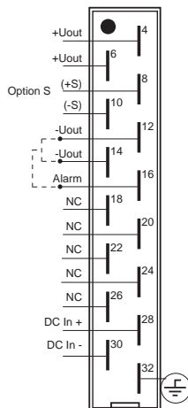
Figure 3. Pin-out DIN41612, H15
