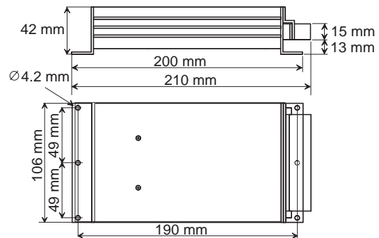
Figure 6. Dimensions with option N, wall mounting Weight: 0.91 kg
